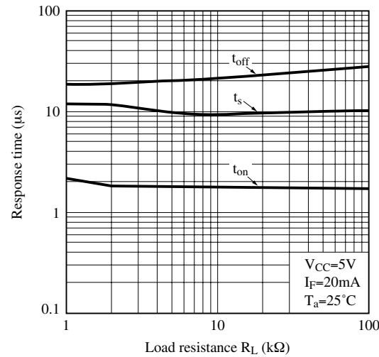
Fig.12 Response Time vs. Load Resistance (saturation region)
